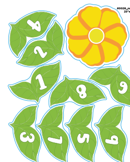
Stem-Numbers 1-9 (#206)
